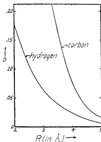
FIG. 7. Vicinal action of carbon and hydrogen atoms
