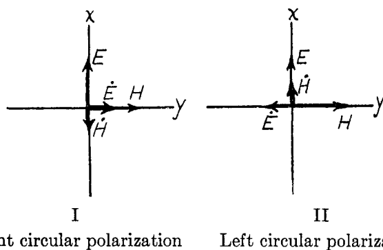
FIG. 1. Electric and magnetic vectors and their time derivatives
