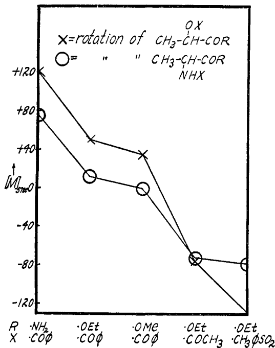
FIG. 20. Comparison of rotation of \text{CH}_3\text{CHOXCOR} and \text{CH}_3\text{CH}(\text{NHX})\text{COR}
